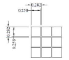
Detail Pixel Scale (10:1)
